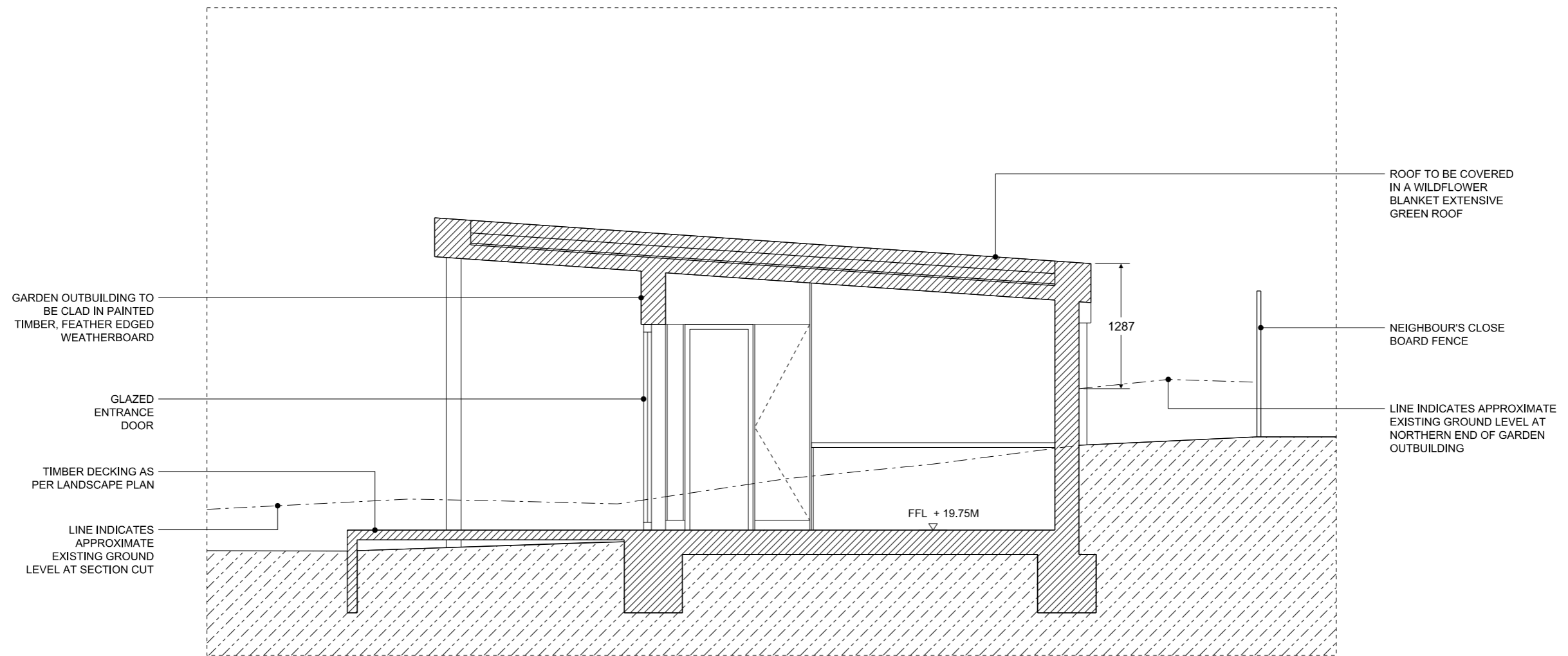
01 GARDEN OUTBUILDING SECTION A3002 1:50 @ A3
